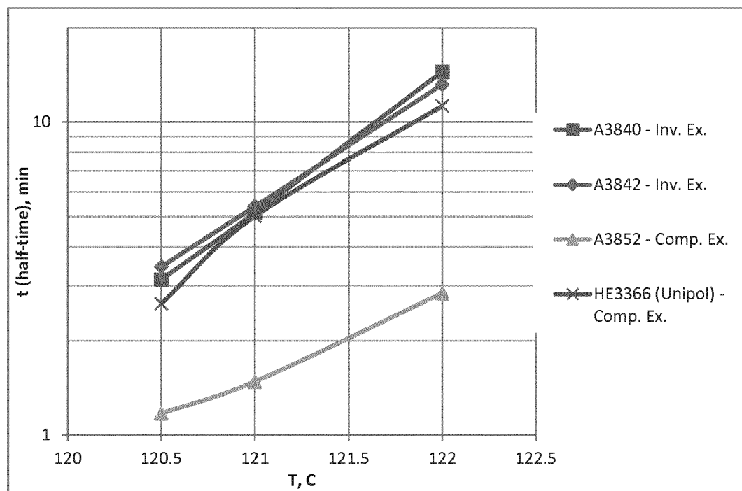
Figure 1. Crystallization half-time at different temp.
