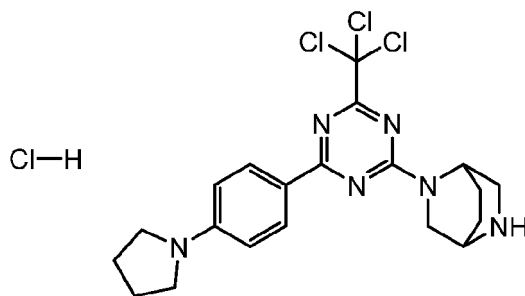
2-(4-(4-(pyrrolidin-1-yl)phenyl)-6-(trichloromethyl)-1,3,5-triazin-2-yl)-2,5-diazabicyclo[2.2.2]octane hydrochloride
