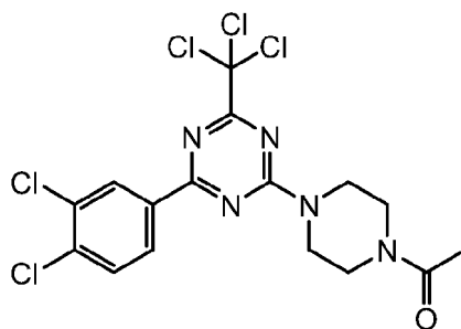
1-(4-(4-(3,4-dichlorophenyl)-6-(trichloromethyl)-1,3,5-triazin-2-yl)piperazin-1-yl)ethan-1-one
