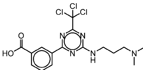
3-(4-((3-(dimethylamino)propyl)amino)-6-(trichloromethyl)-1,3,5-triazin-2-yl)benzoic acid
