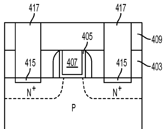
FIG. 4C PRIOR ART
