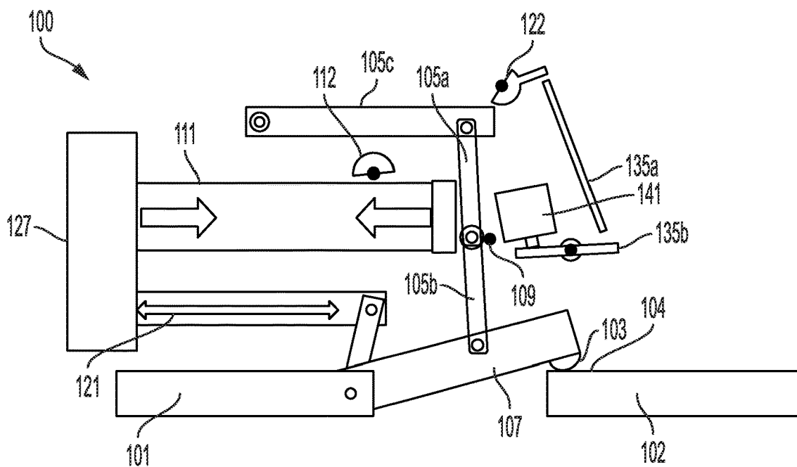
FIG. 1C PRIOR ART
