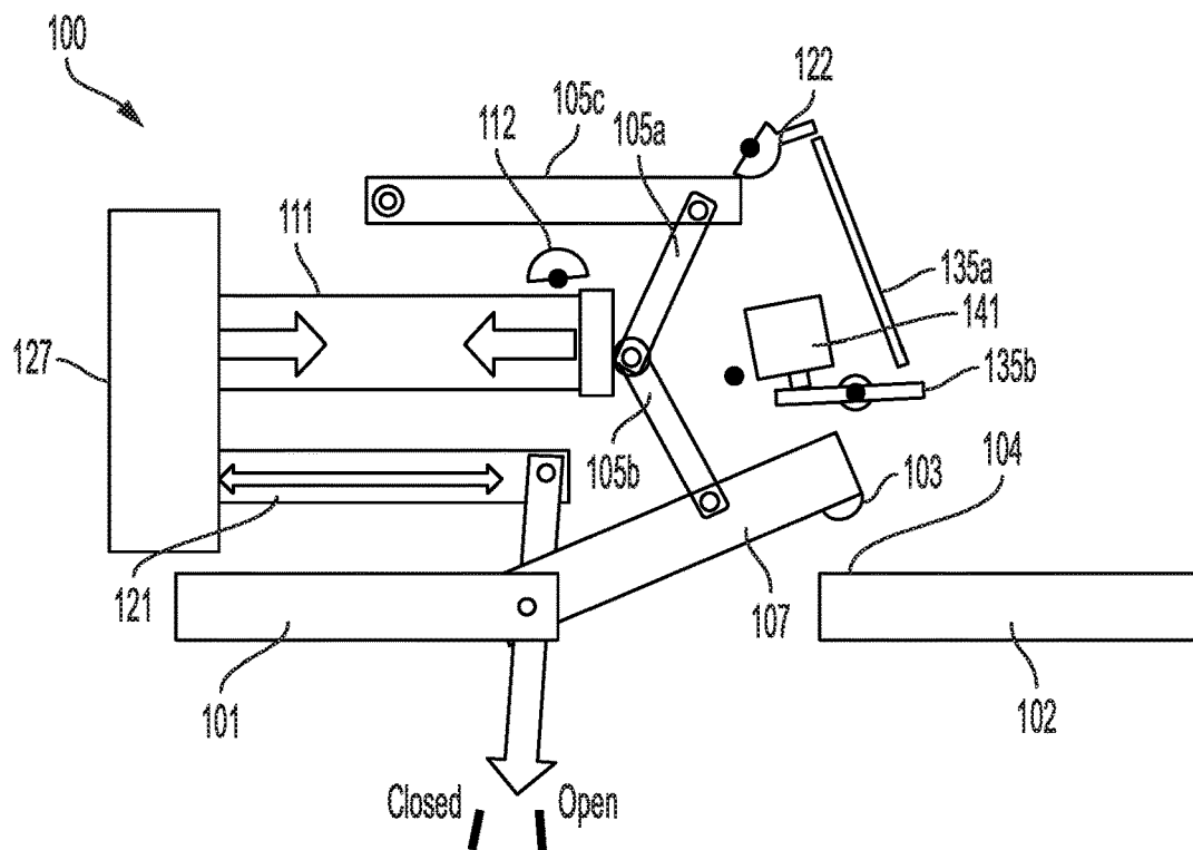
FIG. 1C PRIOR ART
