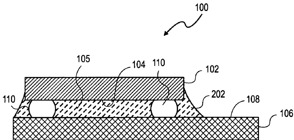
FIG. 2 (PRIOR ART)
