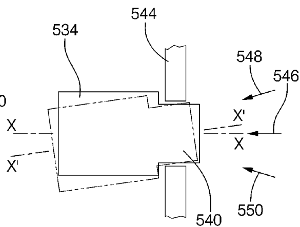
PRIOR ART FIG. 45
