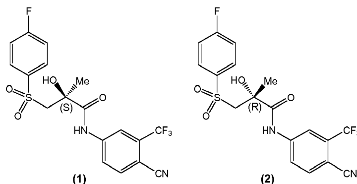
(S)-Bicalutamide (1) and (R)-bicalutamide (2) structures
