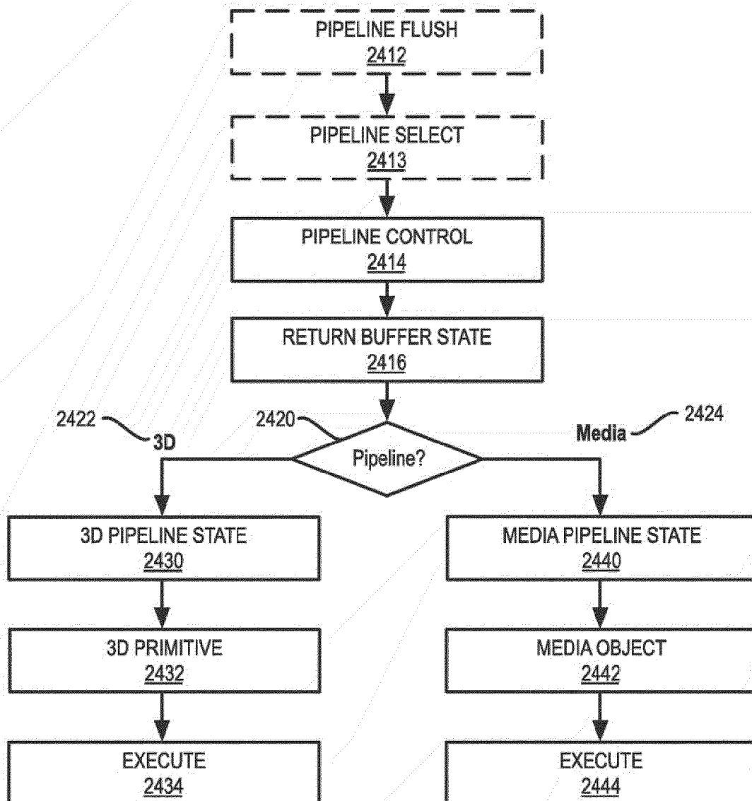
GRAPHICS PROCESSOR COMMAND SEQUENCE 2410
