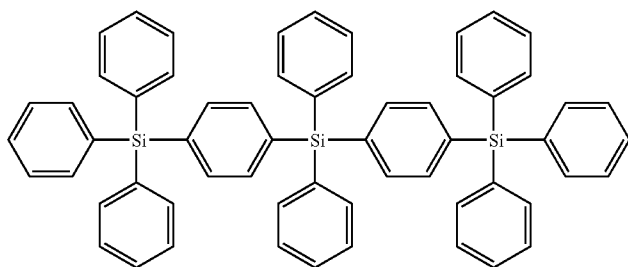
Comparative Compound 3
