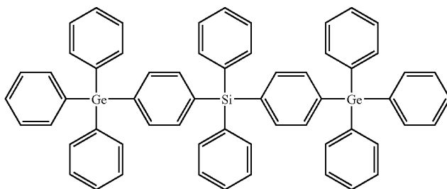
Comparative Compound 4
