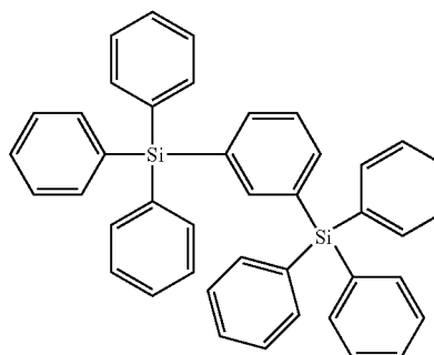
Comparative Compound 1
