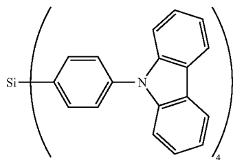
Comparative Compound 2
