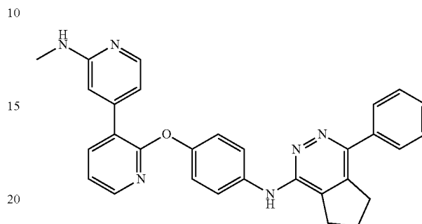
Synthesis of N-(4-(3-(2-(methylamino)pyridin-4-yl)pyridin-2-yloxy)phenyl)-4-phenyl-6,7-dihydro-5H-cyclopenta[d]pyridazin-1-amine
