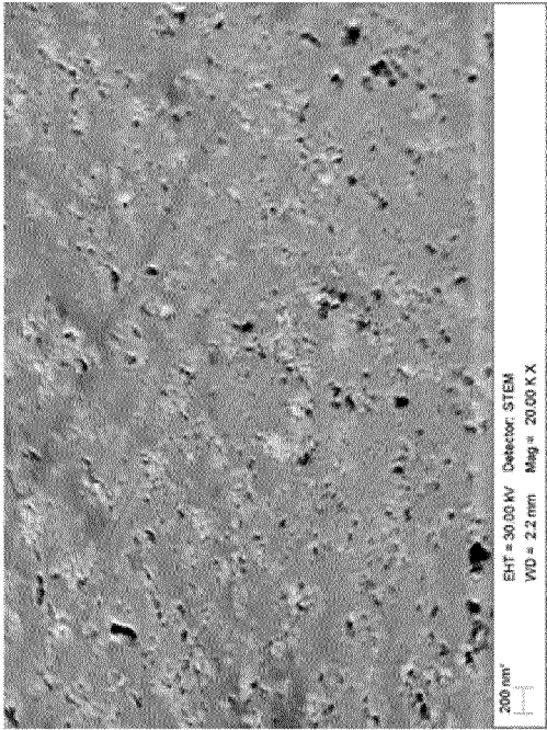
FIG. 7C (Ex1.3, 4.5% siloxane, 20kx)
