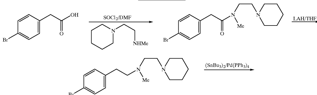
Reaction Scheme IV
