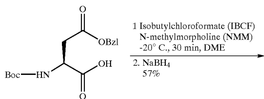
Scheme 5
