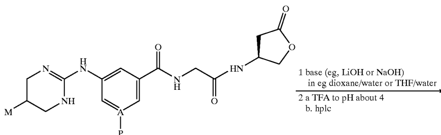
Scheme 8
