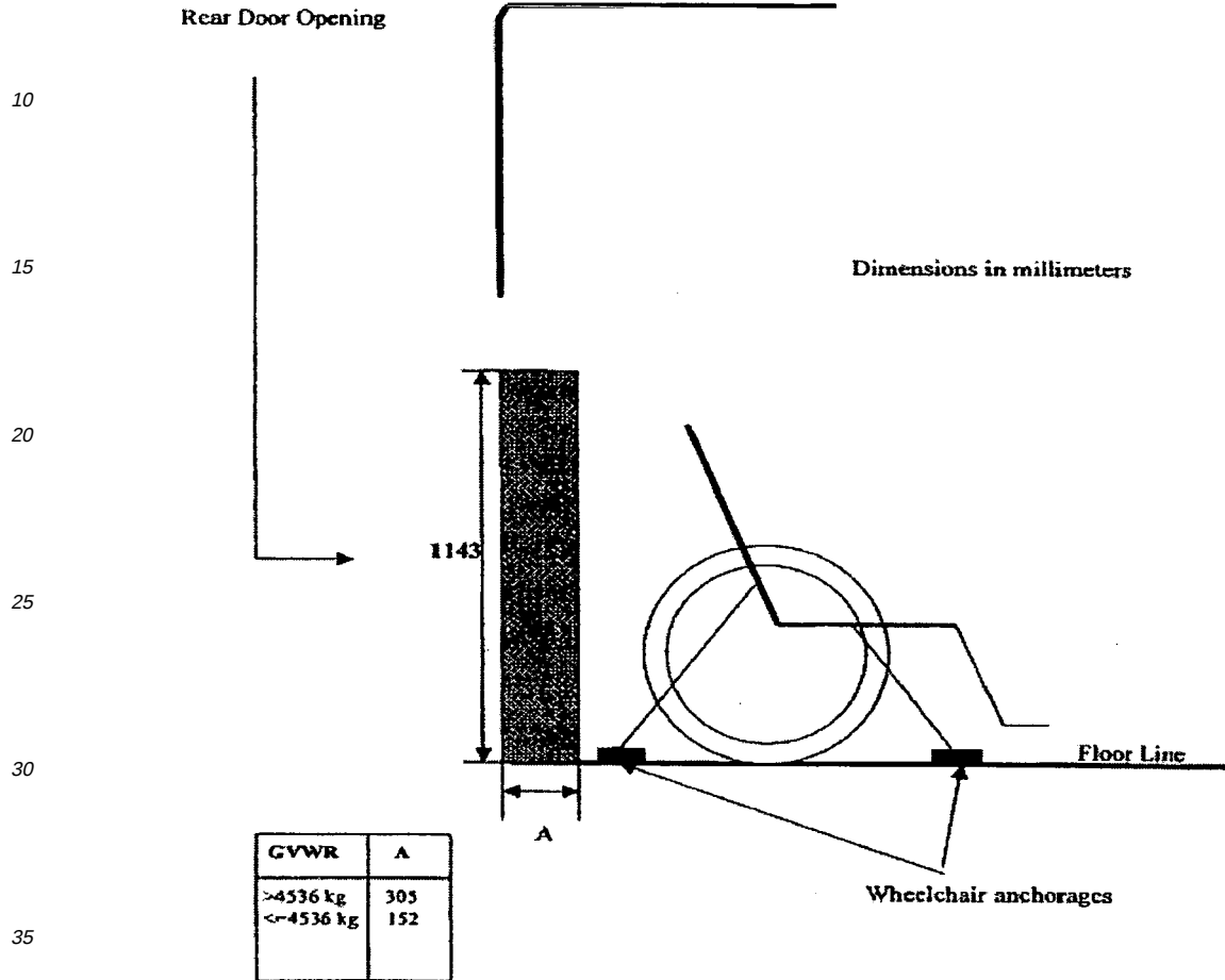
Figure 6 D. Rear Door Emergency Exit - No Wheelchair Anchorages within the shaded region
