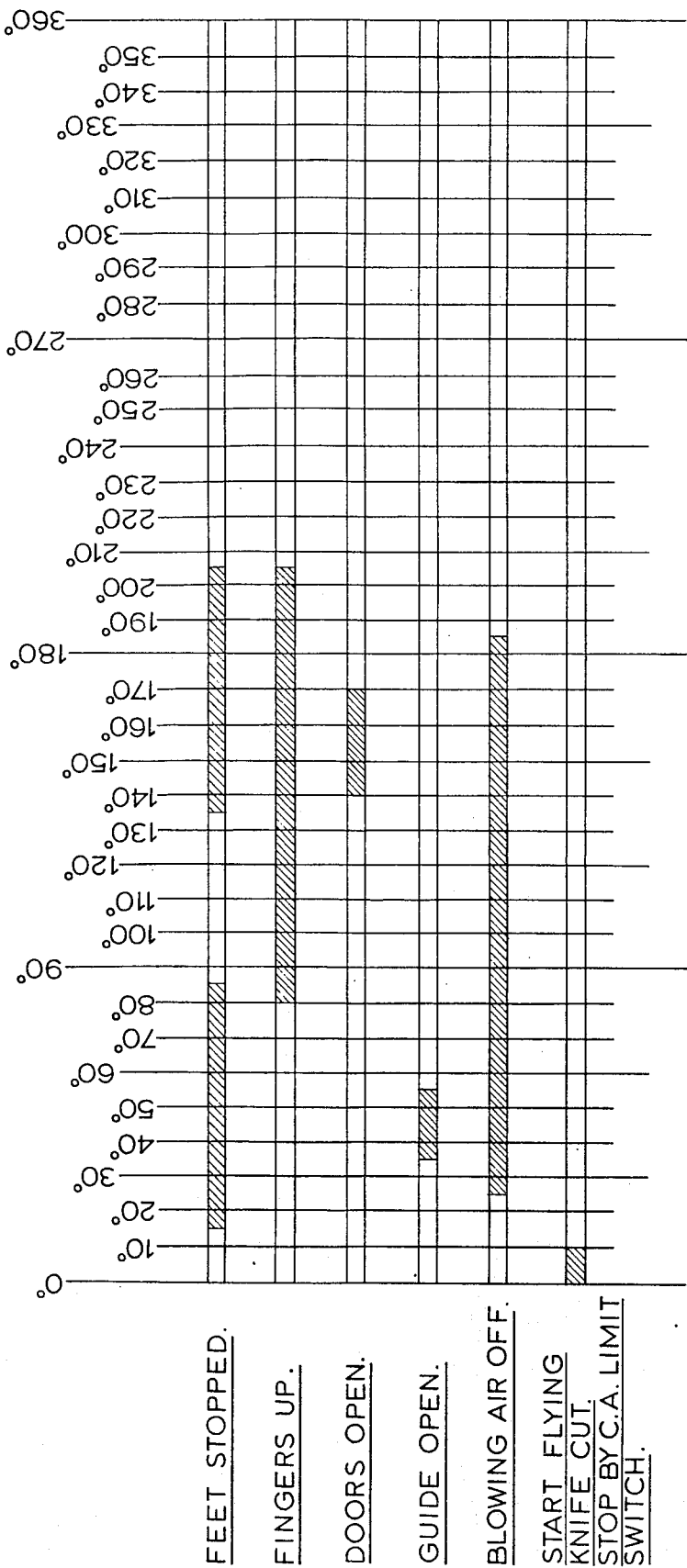
DISCHARGE SEQUENCE : CONTROL BY VARIABLE SPEED CAM TIMER CYCLE TIME DEPENDANT ON SPEED OF FILM FEED (AVERAGE 15 SECS.)
