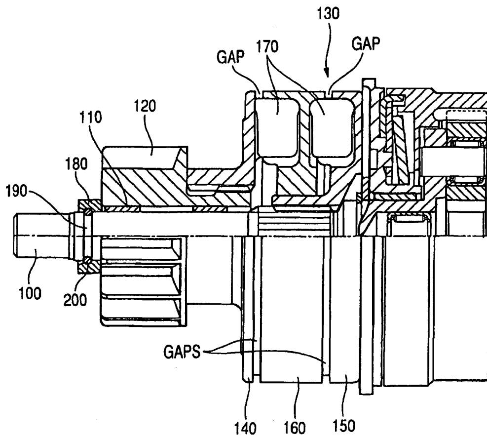
FIG. 5 (RELATED ART)
