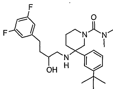
EXAMPLE 244: 3-(3-TERT-BUTYL-PHENYL)-3-[4-(3,5-DIFLUORO-PHENYL)-2-HYDROXY-BUTYLAMINO]-PIPERIDINE-1-CARBOXYLIC ACID DIMETHYLAMIDE
