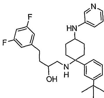
EXAMPLE 234: 1-[1-(3-TERT-BUTYL-PHENYL)-4-(PYRIDIN-3-YLAMINO)-CYCLOHEXYLAMINO]-4-(3,5-DIFLUORO-PHENYL)-BUTAN-2-OL
