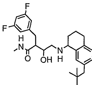
EXAMPLE 152: 2-(3,5-DIFLUORO-BENZYL)-4-[7-(2,2-DIMETHYL-PROPYL)-1,2,3,4-TETRAHYDRO-NAPHTHALEN-1-YLAMINO]-3-HYDROXY-N-METHYL-BUTYRAMIDE
