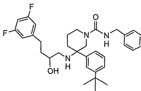
EXAMPLE 246: 3-(3-TERT-BUTYL-PHENYL)-3-[4-(3,5-DIFLUORO-PHENYL)-2-HYDROXY-BUTYLAMINO]-PIPERIDINE-1-CARBOXYLIC ACID ISOPROPYLAMIDE
