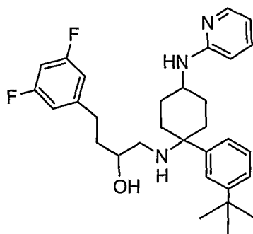
EXAMPLE 236: 1-[1-(3-TERT-BUTYL-PHENYL)-4-TRIFLUOROMETHYL-CYCLOHEXYLAMINO]-4-(3,5-DIFLUORO-PHENYL)-BUTAN-2-OL
