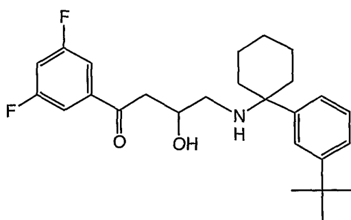
EXAMPLE 143: 4-[1-(3-TERT-BUTYL-PHENYL)-CYCLOHEXYLAMINO]-1-(3,5-DIFLUORO-PHENYL)-3-HYDROXY-BUTAN-1-ONE
