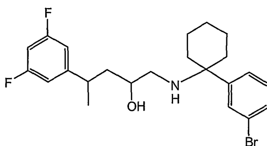
EXAMPLE 150: 1-[1-(3-BROMO-PHENYL)-CYCLOHEXYLAMINO]-4-(3,5-DIFLUORO-PHENYL)-PENTAN-2-OL
