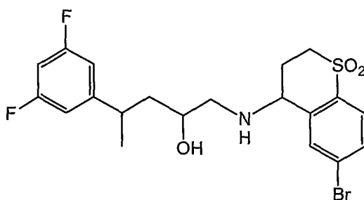
EXAMPLE 145: 1-(6-BROMO-1,1-DIOXO-1 \lambda^6 -THIOCHROMAN-4-YLAMINO)-4-(3,5-DIFLUORO-PHENYL)-4-METHYLAMINO-BUTAN-2-OL
