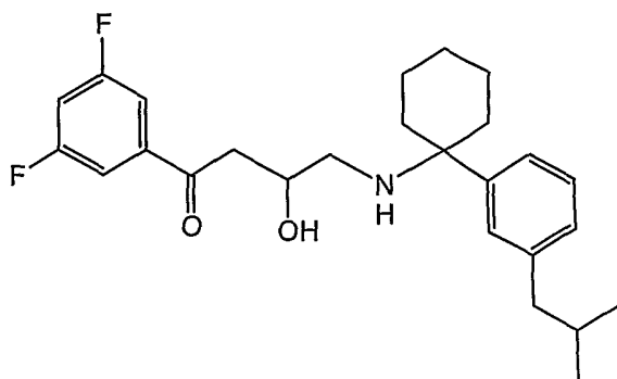
EXAMPLE 143: 4-[1-(3-TERT-BUTYL-PHENYL)-CYCLOHEXYLAMINO]-1-(3,5-DIFLUORO-PHENYL)-3-HYDROXY-BUTAN-1-ONE
