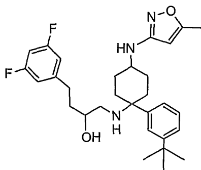
EXAMPLE 234: 1-[1-(3-TERT-BUTYL-PHENYL)-4-(PYRIDIN-3-YLAMINO)-CYCLOHEXYLAMINO]-4-(3,5-DIFLUORO-PHENYL)-BUTAN-2-OL
