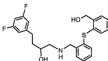
EXAMPLE 196: 4-(3,5-DIFLUORO-PHENYL)-1-[2-(2-HYDROXYMETHYL-PHENYLSULFANYL)-BENZYLAMINO]-BUTAN-2-OL
