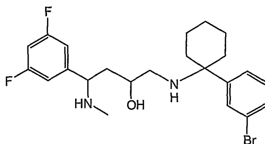
EXAMPLE 151: 1-[1-(3-BROMO-PHENYL)-CYCLOHEXYLAMINO]-4-(3,5-DIFLUORO-PHENYL)-4-METHYLAMINO-BUTAN-2-OL
