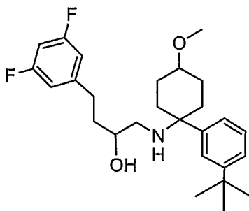
EXAMPLE 228: 4-(3-TERT-BUTYL-PHENYL)-4-[4-(3,5-DIFLUORO-PHENYL)-2-HYDROXY-BUTYLAMINO]-CYCLOHEXANONE
