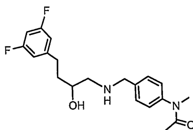
EXAMPLE 197: N-(4-([4-(3,5-DIFLUORO-PHENYL)-2-HYDROXY-BUTYLAMINO]-METHYL)-PHENYL)-N-METHYL-ACETAMIDE
