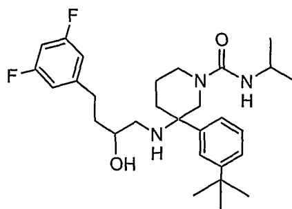
EXAMPLE 246: 3-(3-TERT-BUTYL-PHENYL)-3-[4-(3,5-DIFLUORO-PHENYL)-2-HYDROXY-BUTYLAMINO]-PIPERIDINE-1-CARBOXYLIC ACID ISOPROPYLAMIDE
