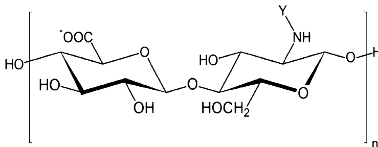
Formula Ib
