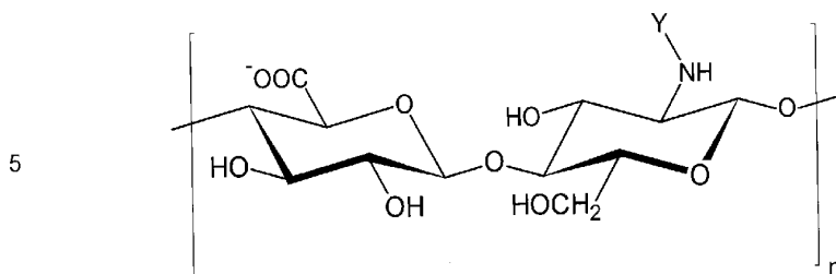
Formula Ib
