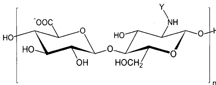
Formula Ib
