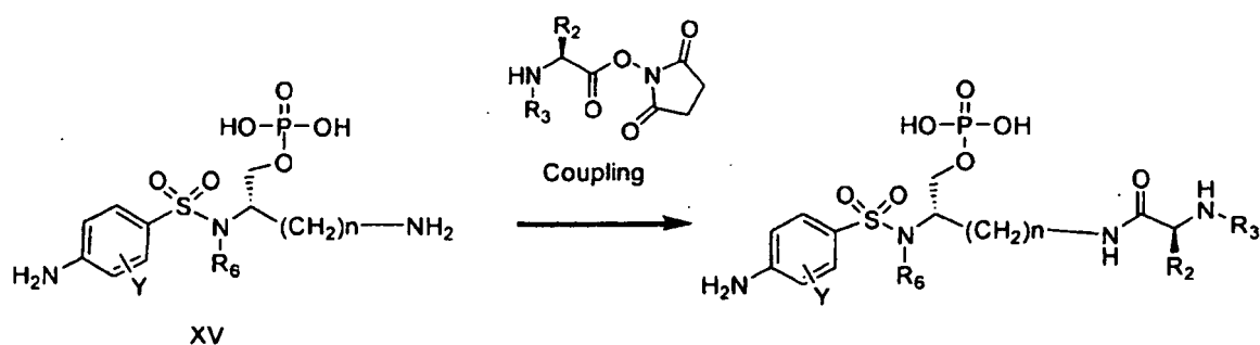
Scheme 2D
