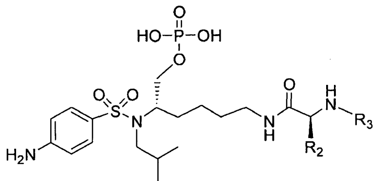
III
