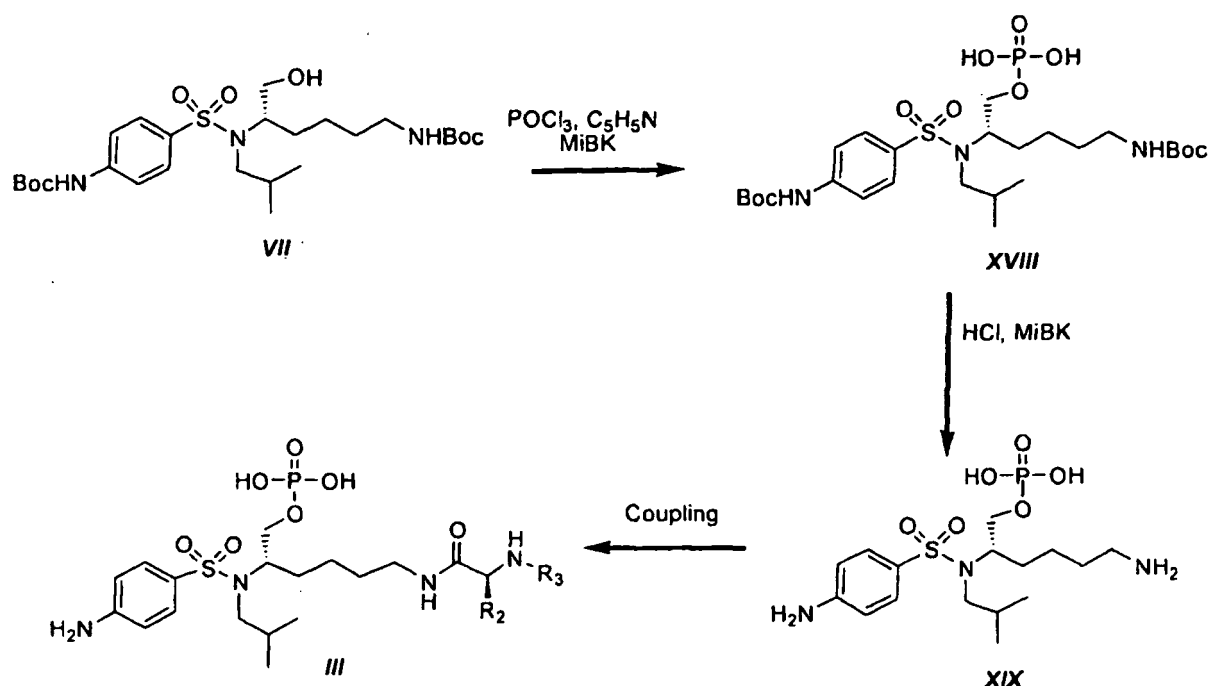
Scheme 2B
