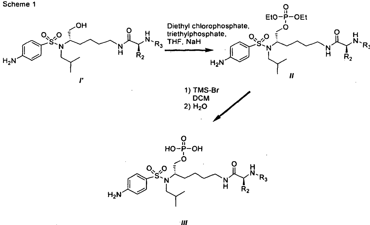
Scheme 1
