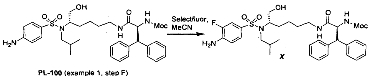
Scheme 3
