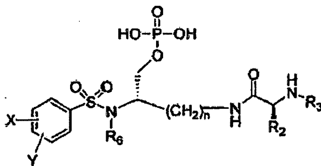
IIIA
