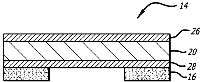
FIG. 3 (Prior Art)
