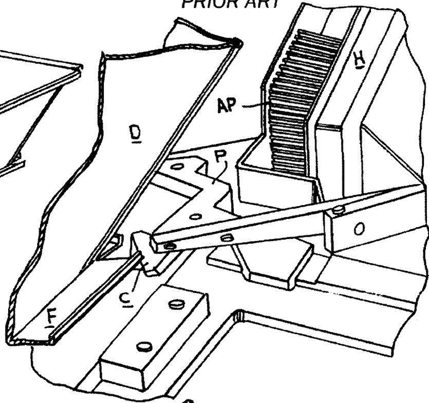
FIG. 2 PRIOR ART
