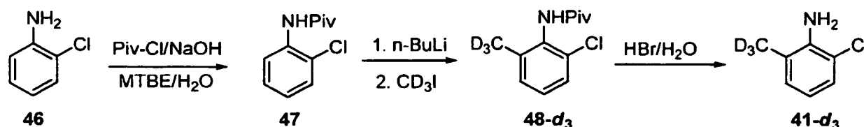
Scheme 1. Preparation of Intermediate 41-d_3 .
