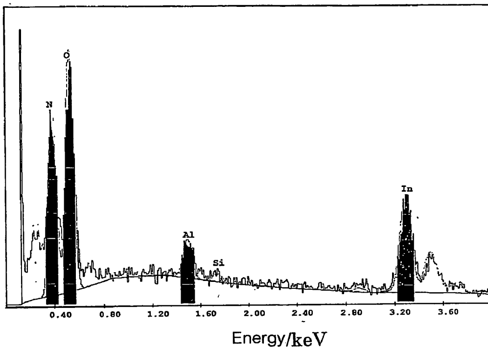
EDX spectrum of oxinitride material
