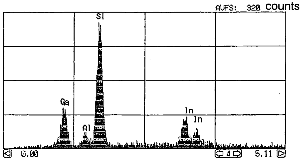
( b ) Composition analysis pattern of GaAlInN by EDX
