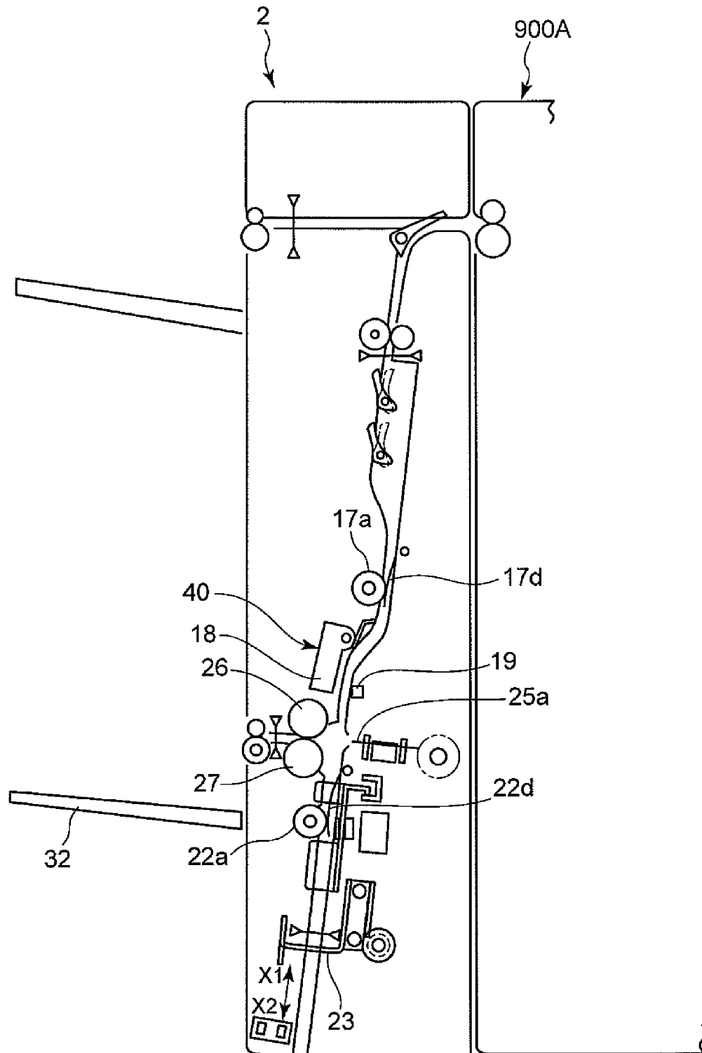
FIG. 18 PRIOR ART
