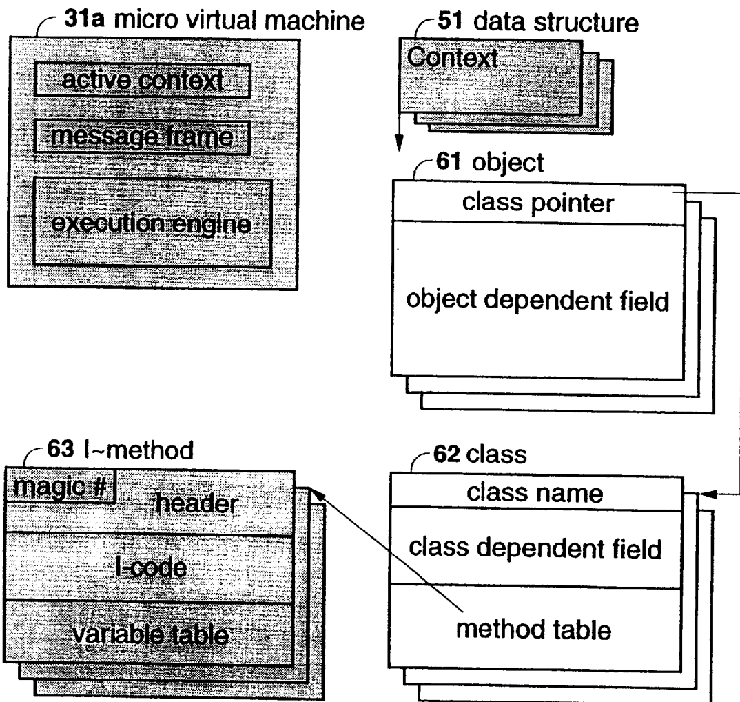
overall structure of MVM
