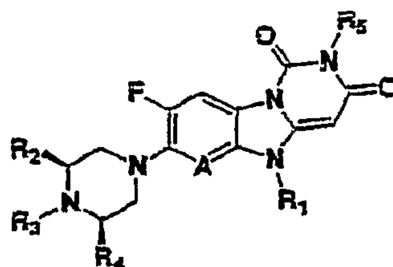
Pyrimido[1,6-a]benzimidazoles'
