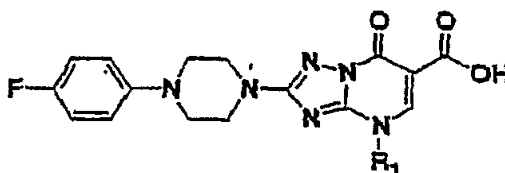
2-[4-(4-Fluorophenyl)piperizin-1-yl]-4,7-dihydro-7-oxo-1,2,4-triazolo[1,5-a]pyrimidine-6-carboxylic Acids
