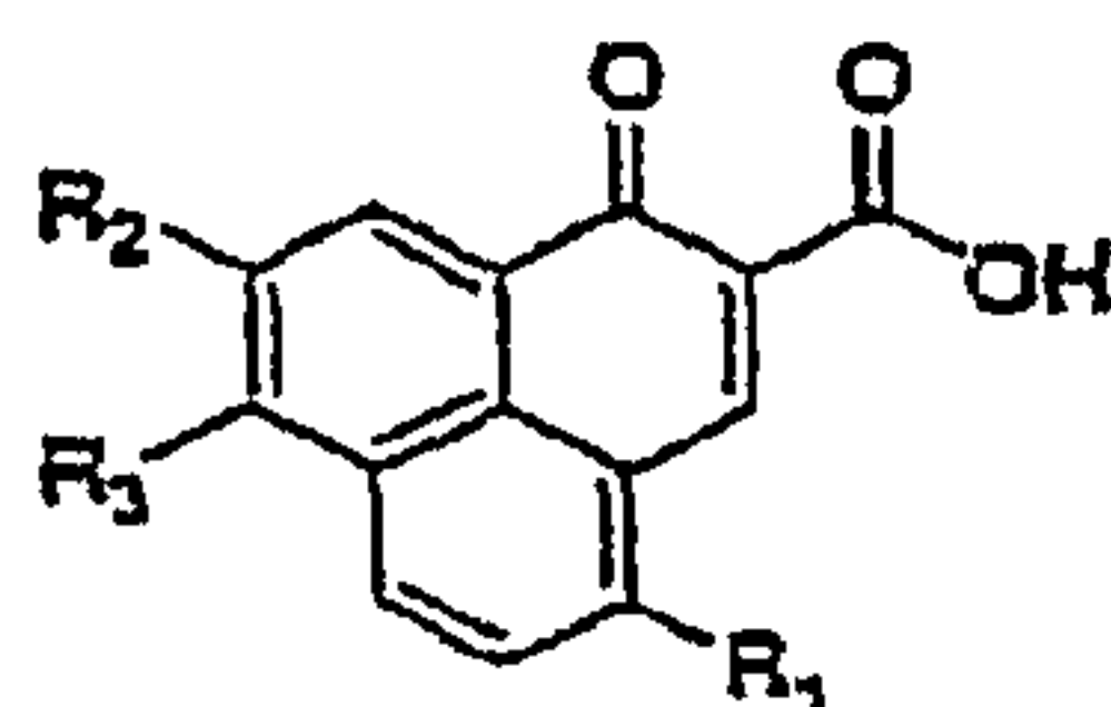
p-Quinone Methides
