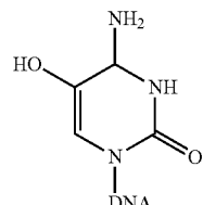
5-hydroxycytosine
