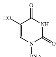
5-hydroxyuracil
