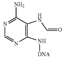
4,6-diamino-5-formamidopyrimidine (Fapy-adenine)
