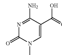
5-carboxycytosine
