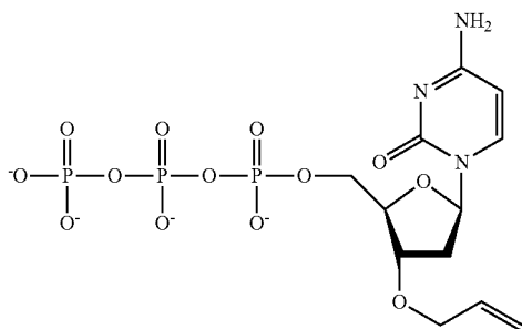
3'-O-allyl-dCTP:
