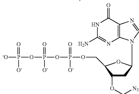
3'-O-azidomethyl-dGTP
