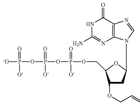
3'-O-allyl-dGTP:
