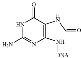
2,6-diamino-4-hydroxy-5-formamidopyrimidine (Fapy-guanine)
