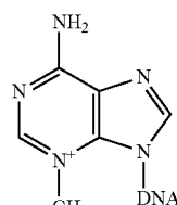
3-methyladenine
