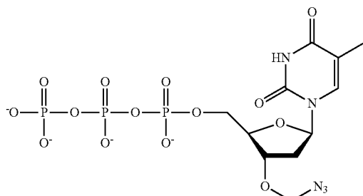
3'-O-azidomethyl-dTTP
