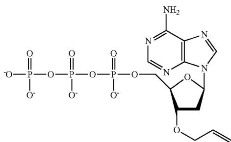
3'-O-allyl-dATP:
