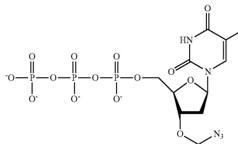
3'-O-azidomethyl-dTTP:
