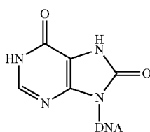
7,8-dihydro-8-oxo-nebularine
