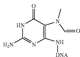
2,6-diamino-4-hydroxy-5-N-methylformamidopyrimidine
