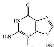
3-methylguanine
