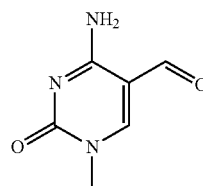
5-formylcytosine
