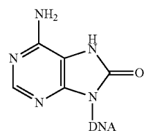
7,8-dihydro-8-oxo-adenine
