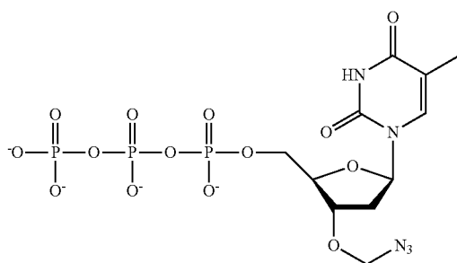
3'-O-azidomethyl-dTTP
