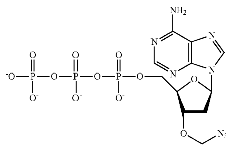
3'-O-azidomethyl-dATP:
