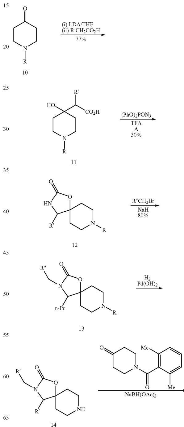
SCHEME 1
