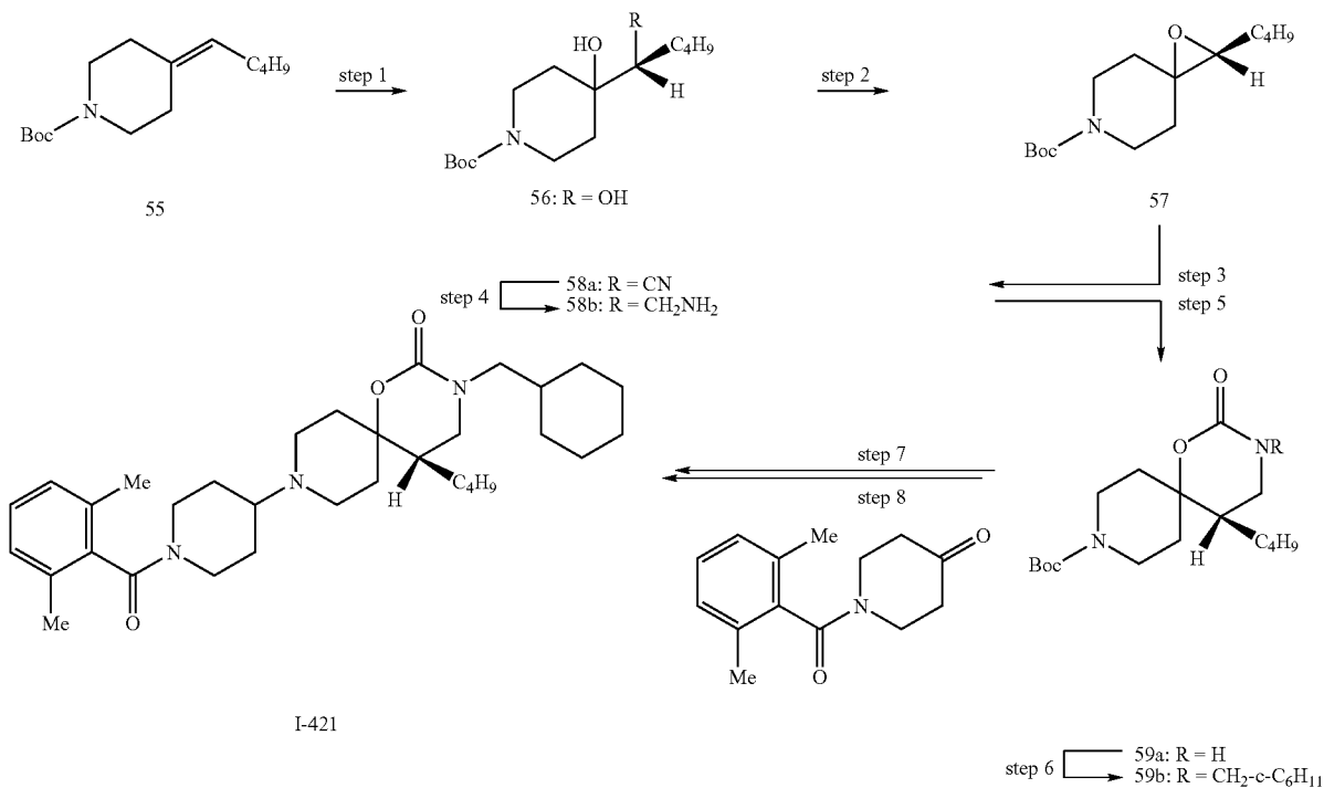
SCHEME 8
