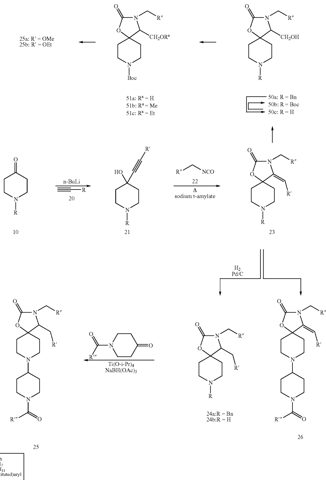
SCHEME 4
