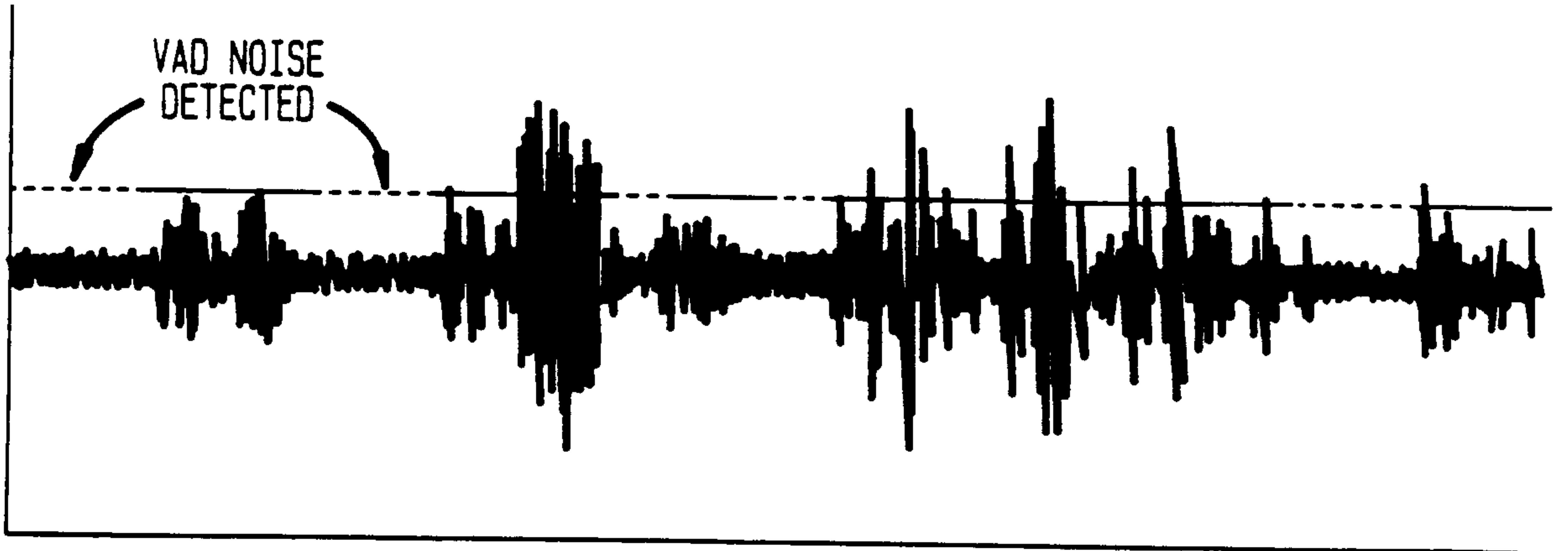
FIG. 8 INPUT SIGNAL & NOISE
