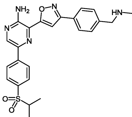
Compound A.
