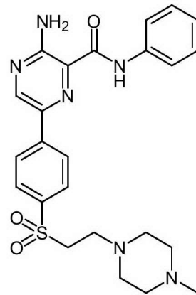
Compound 3
