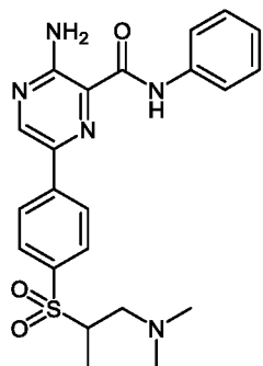
Compound 1
