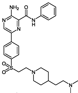
Compound 5
