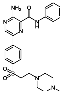
Compound 3
