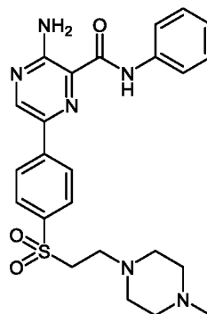
Compound 3
