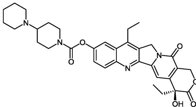
Irinotecan
