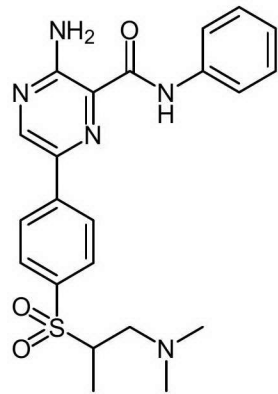
Compound 1
