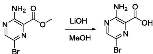
Intermediate 6
