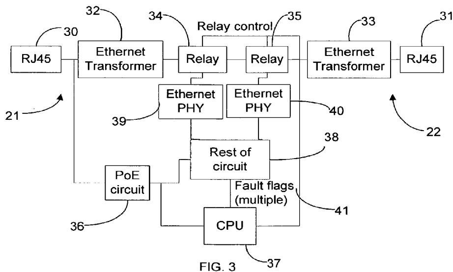
Device with Fail over Bypass
