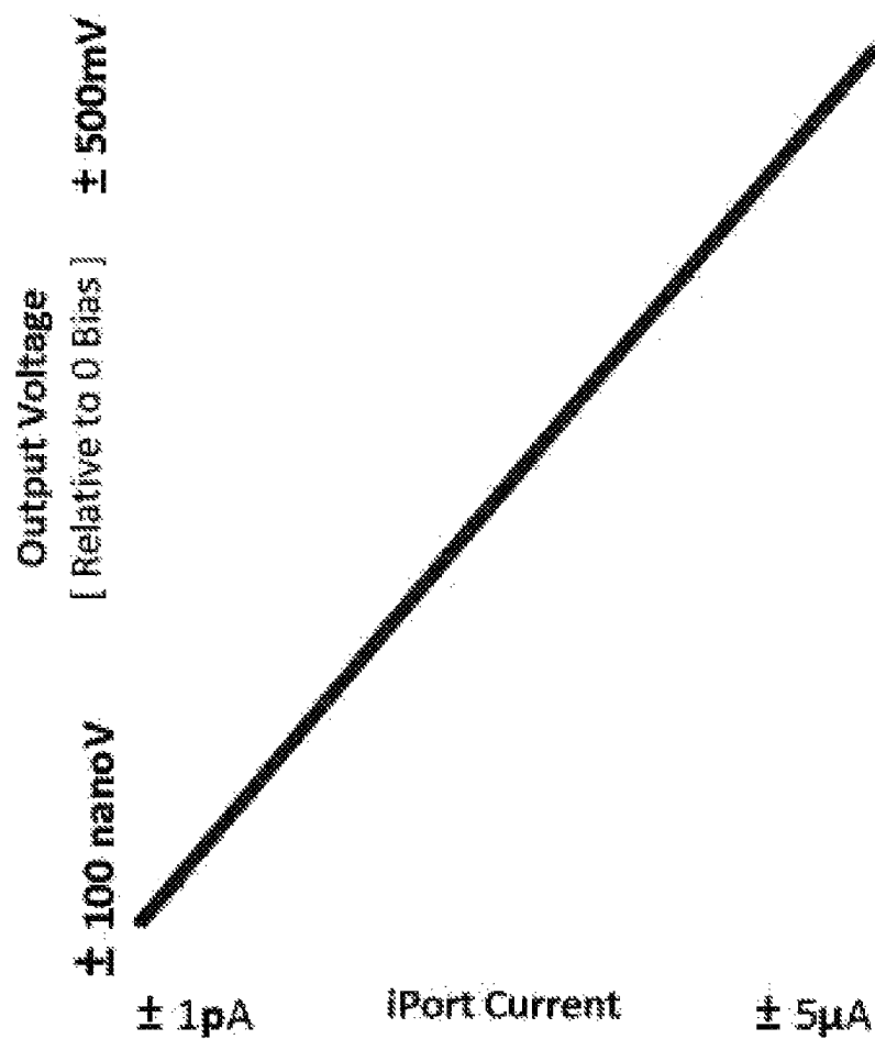
Fig.3h CiFET Transfer Properties \equiv LINEAR Trans-Resistance
