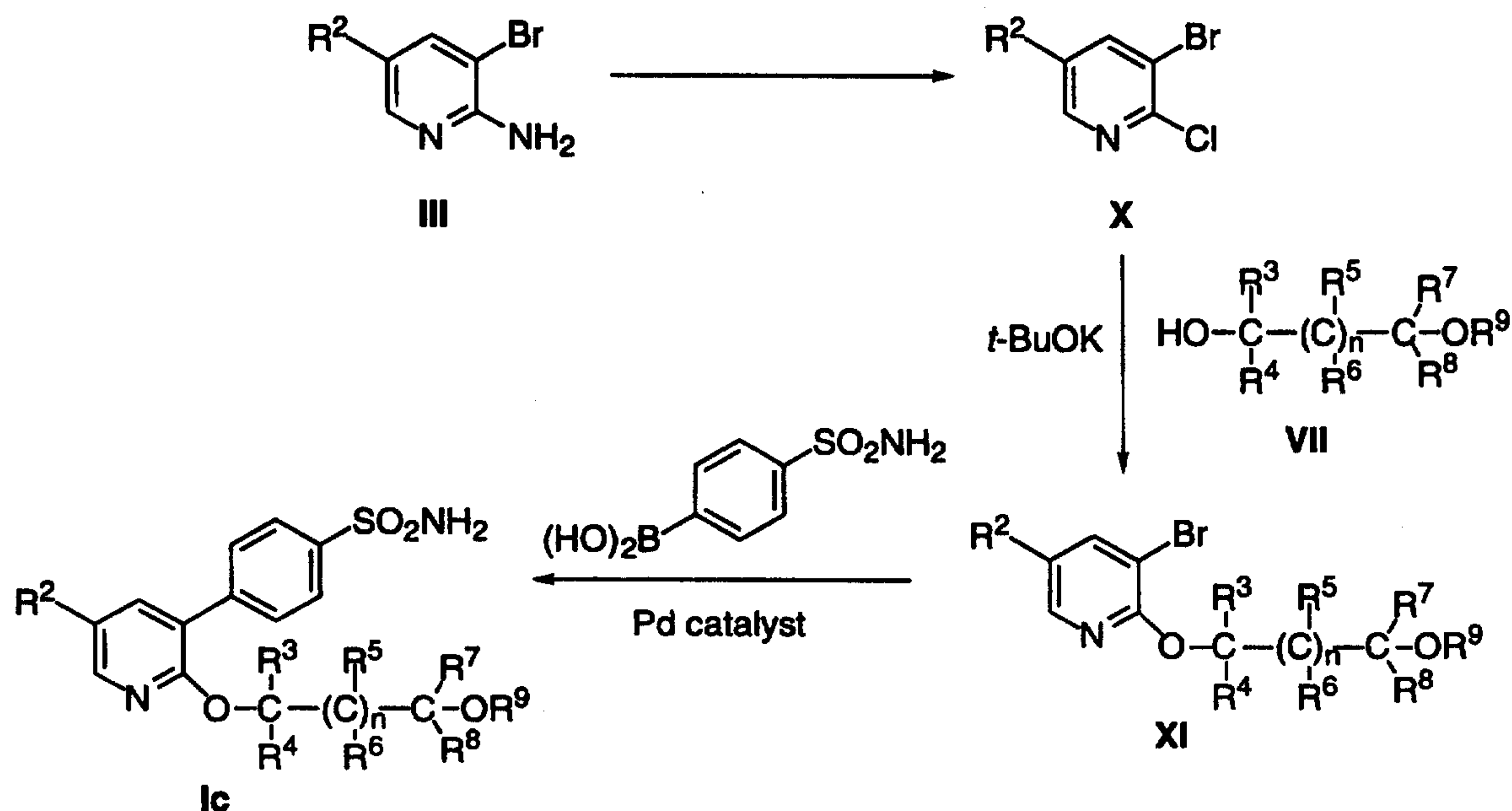
SCHEME 4
