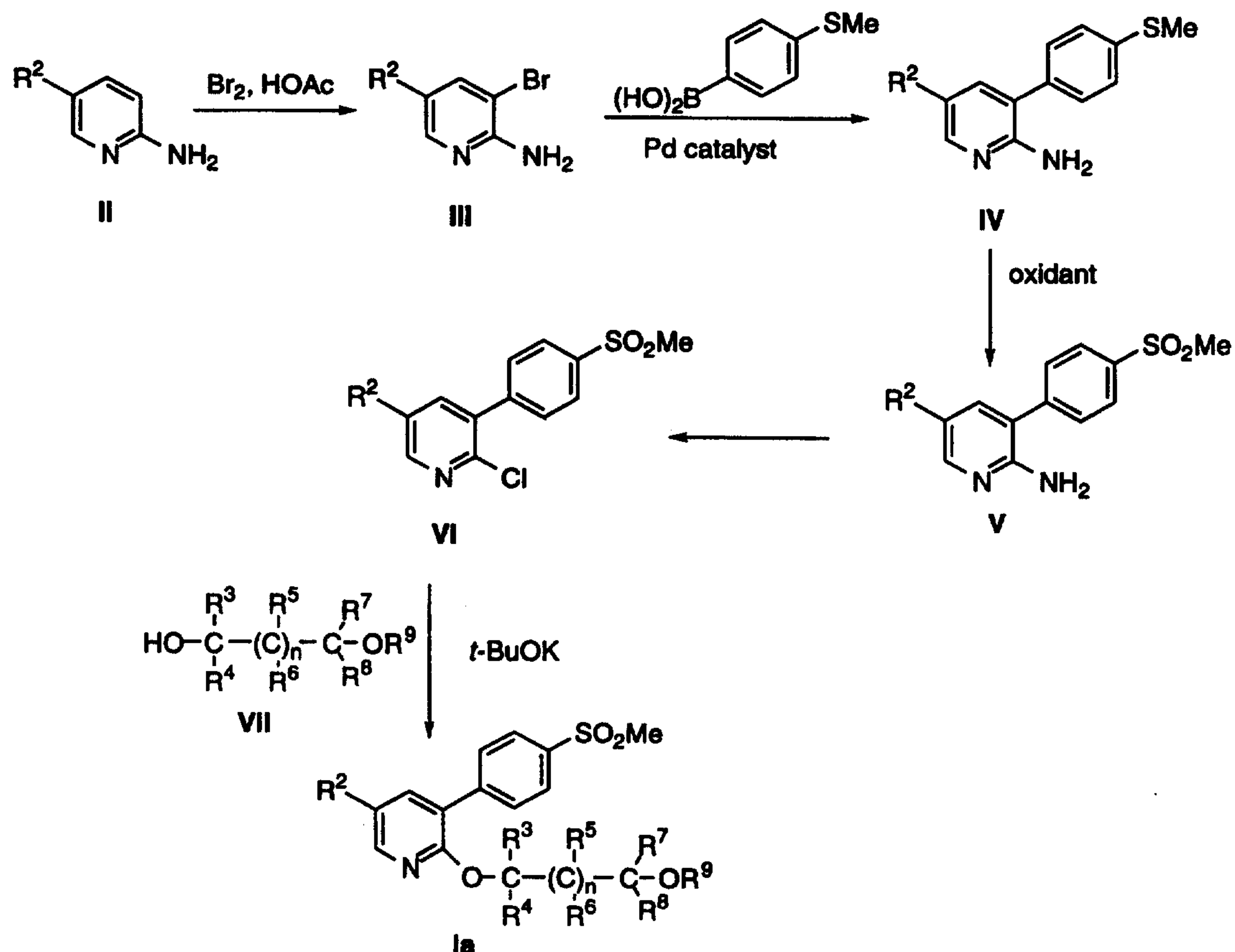
SCHEME 2
