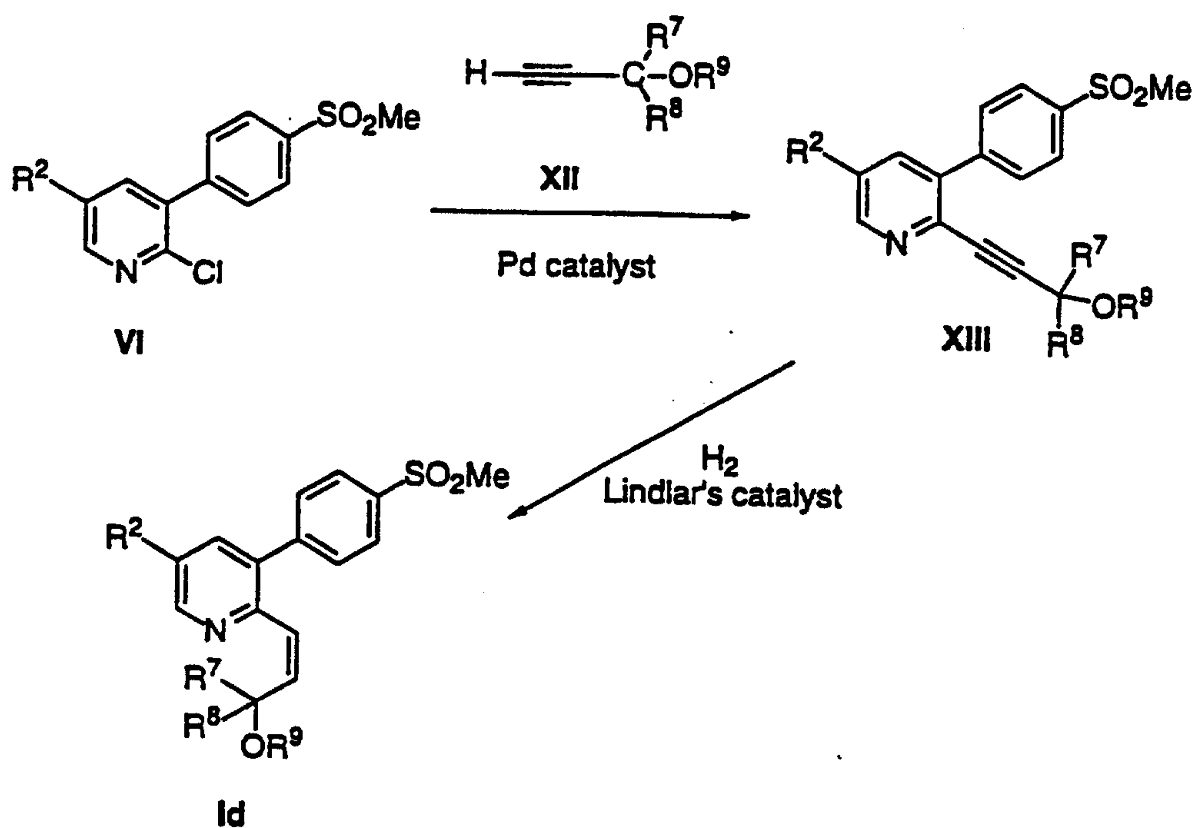
Scheme 4
