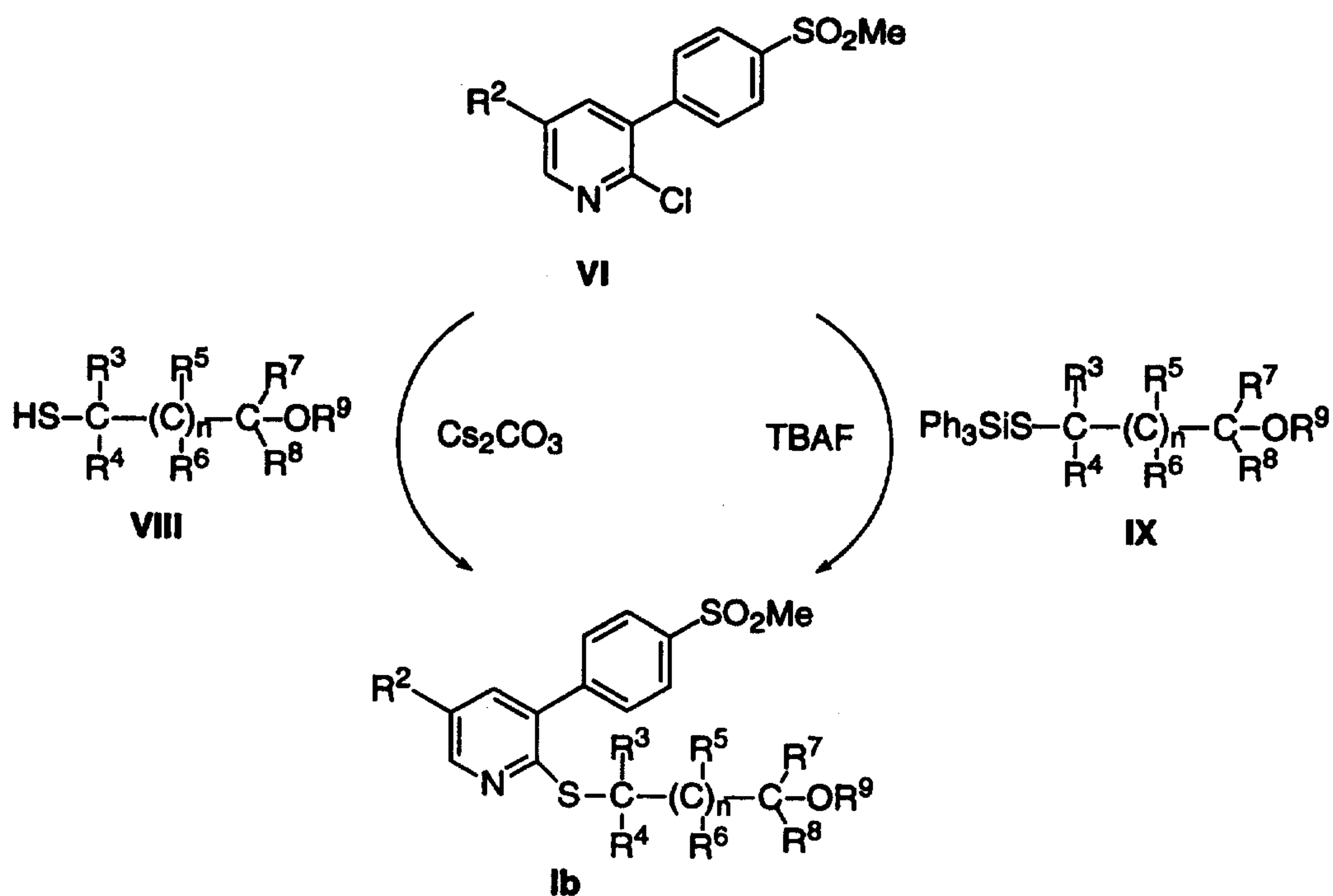
SCHEME 3
