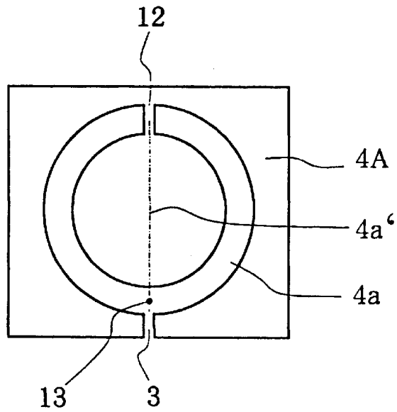
FIG. 2 (PRIOR ART)
