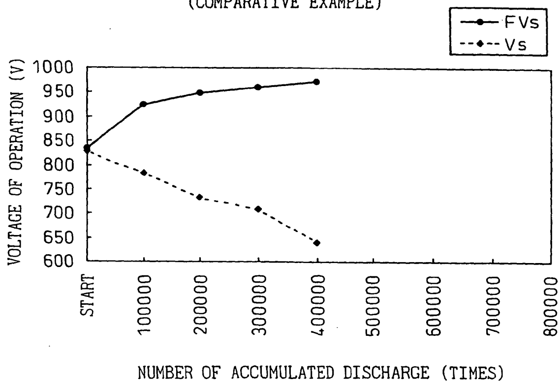
Fig.10 (COMPARATIVE EXAMPLE)
