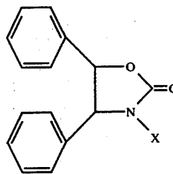
Compound 55
