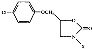
Compound 17
