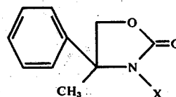
Compound 57
