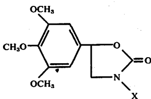
Compound 52
