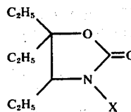
Compound 54
