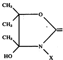
Compound 35
