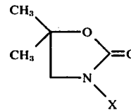
Compound 23
