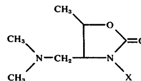
Compound 26
