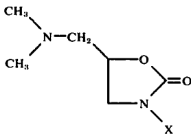
5-[(Dimethylamino)methyl]-N-halo-oxazolidinone
