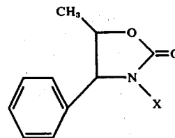
Compound 57
