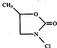
Compound 6
