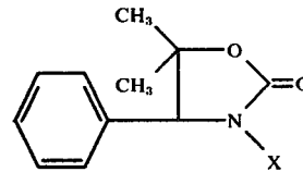
Compound 24
