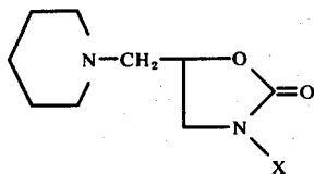
Compound 49
