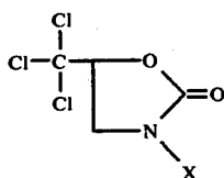
Compound 51
