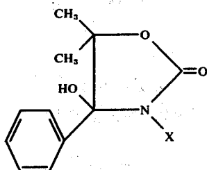
Compound 32
