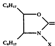
Compound 25
