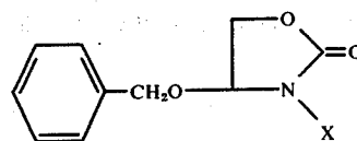
Compound 12
