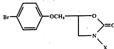
Compound 14
