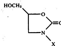
Compound 33
