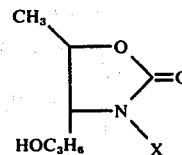
Compound 56
