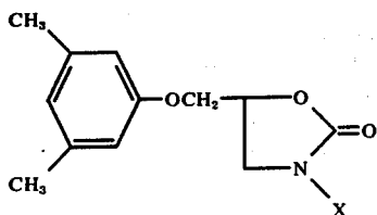
Compound 53
