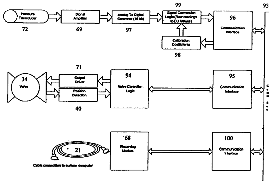
Figure 7 - Downhole Tool Software & Electronics
