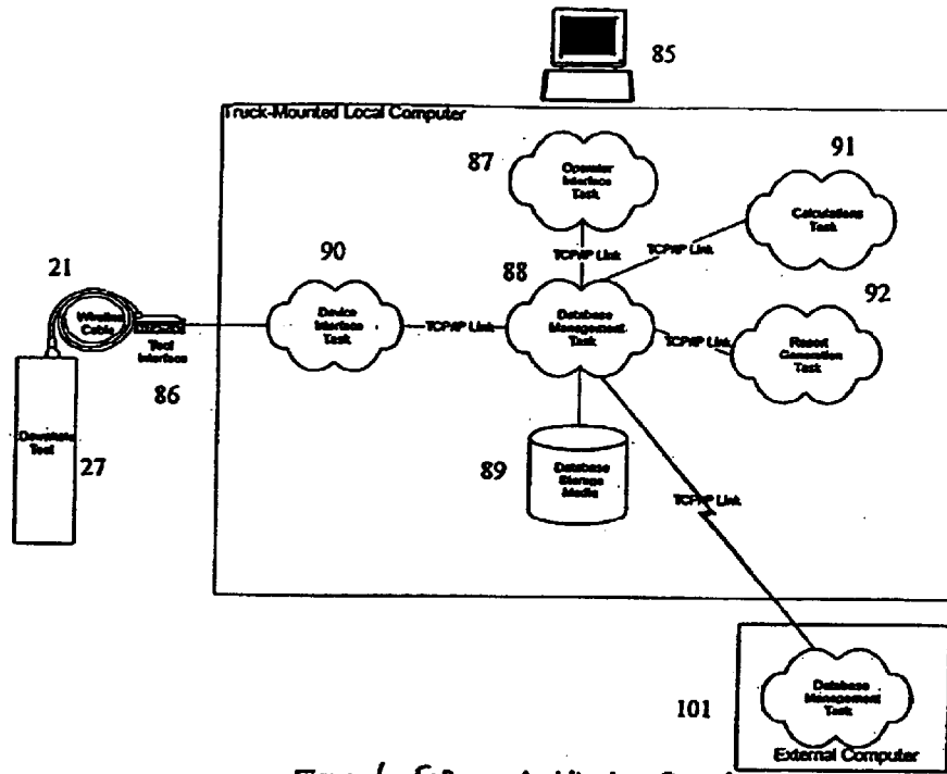
Figure 6 Software Architecture Overview
