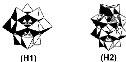
[Chemical Formula 118]
