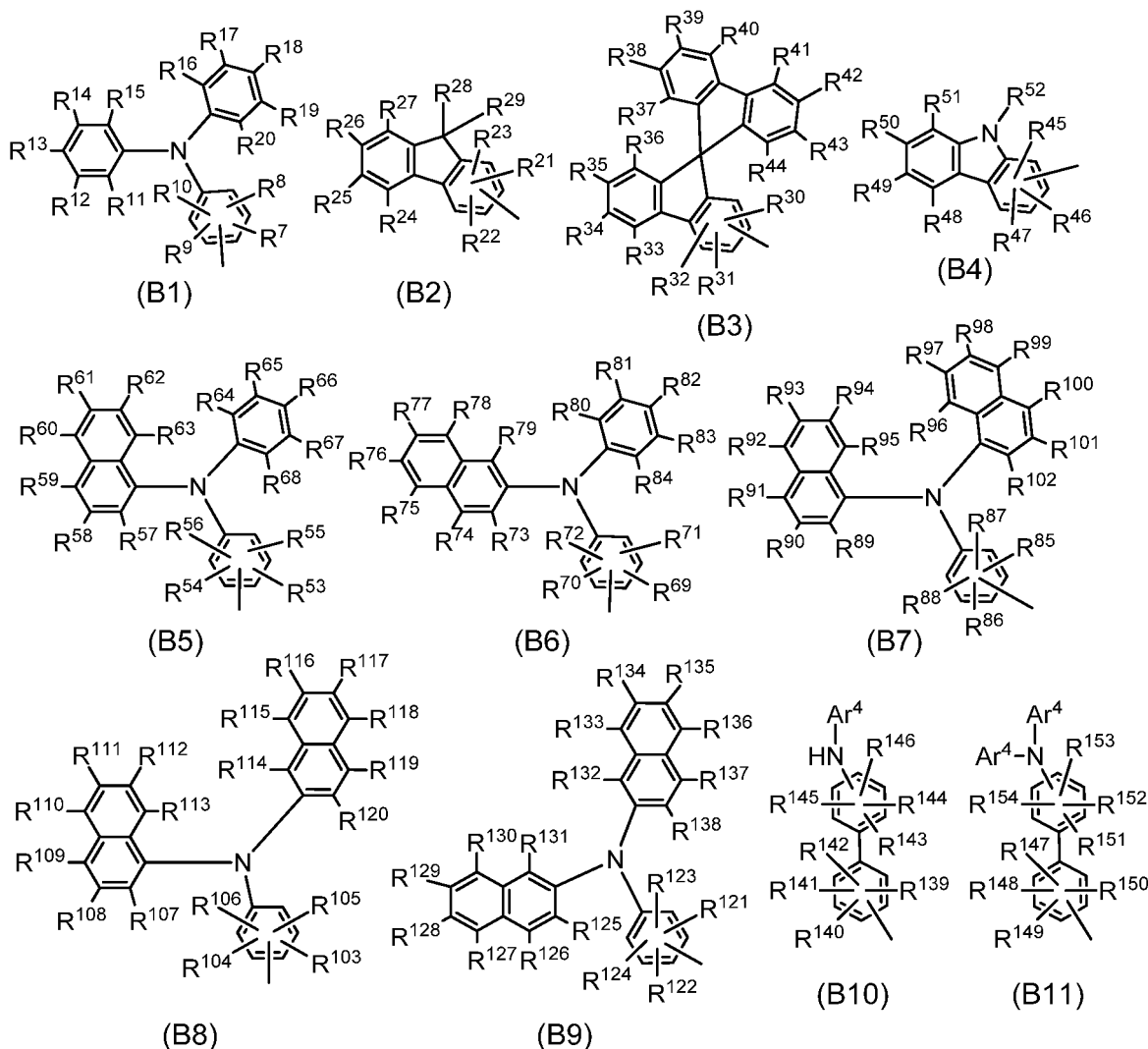
[Chemical Formula 62]
