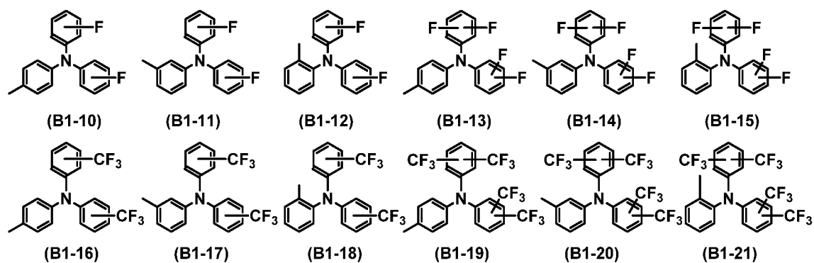
[Chemical Formula 66]
