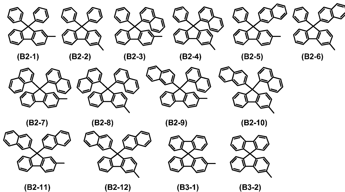
[Chemical Formula 66]
