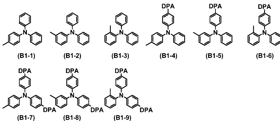
[Chemical Formula 64]
