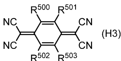
[Chemical Formula 119]
