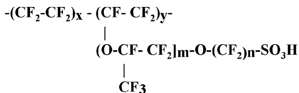
Typical Structure of PFSA Ionomer
