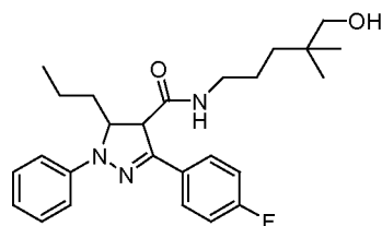
(Compound 4)
