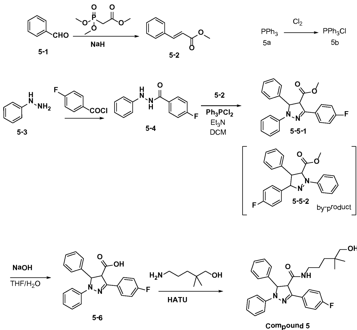
Synthesis Scheme 5
