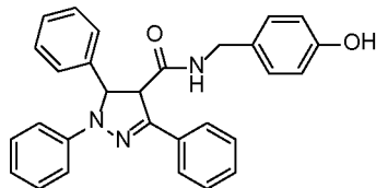
(Compound 2)
