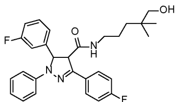
(Compound 6)
