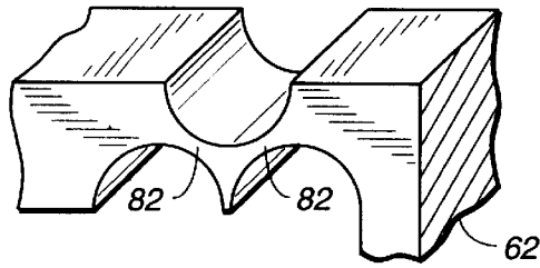
FIG. 4 (PRIOR ART)
