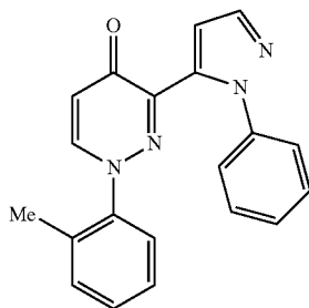
1-(2-Methylphenyl)-3-(1-phenyl-1H-pyrazol-5-yl)pyridazin-4(1H)-one
