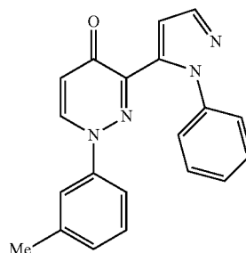
1-(3-Methylphenyl)-3-(1-phenyl-1H-pyrazol-5-yl)pyridazin-4(1H)-one
