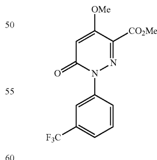
Methyl 4-methoxy-6-oxo-1-[3-(trifluoromethyl)phenyl]-1,6-dihydropyridazine-3-carboxylate
