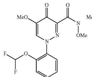
1-[2-(Difluoromethoxy)phenyl]-N,5-dimethoxy-N-methyl-4-oxo-1,4-dihydropyridazine-3-carboxamide
