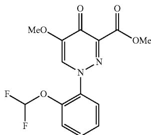
Methyl 1-[2-(difluoromethoxy)phenyl]-5-methoxy-4-oxo-1,4-dihydropyridazine-3-carboxylate
