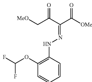
Methyl 2-[[2-(difluoromethoxy)phenyl]hydrazono]-4-methoxy-3-oxobutanoate
