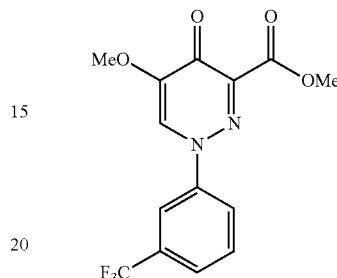
Methyl 5-methoxy-4-oxo-1-[3-(trifluoromethyl)phenyl]-1,4-dihydropyridazine-3-carboxylate
