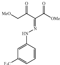
Methyl 4-methoxy-3-oxo-2-{[3-(trifluoromethyl)phenyl]hydrazono}butanoate
