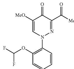
3-Acetyl-1-[2-(difluoromethoxy)phenyl]-5-methoxy-pyridazin-4(1H)-one
