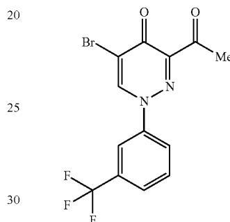
3-Acetyl-5-bromo-1-[3-(trifluoromethyl)phenyl]pyridazin-4(1H)-one
