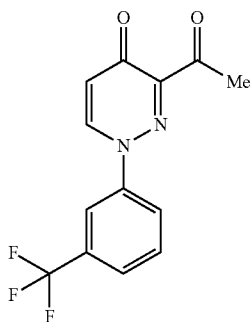
3-Acetyl-1-[3-(trifluoromethyl)phenyl]pyridazin-4(1H)-one
