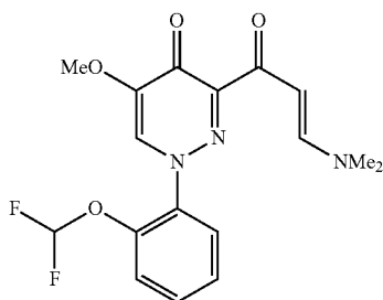
1-[2-(Difluoromethoxy)phenyl]-3-[3-(dimethylamino)prop-2-enyl]-5-methoxypyridazin-4(1H)-one
