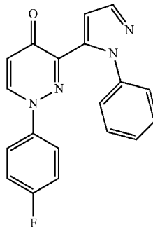
1-(4-Fluorophenyl)-3-(1-phenyl-1H-pyrazol-5-yl) pyridazin-4(1H)-one
