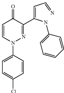
1-(4-Chlorophenyl)-3-(1-phenyl-1H-pyrazol-5-yl)pyridazin-4(1H)-one
