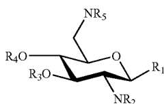
Scaffold W3 derived from C-1
