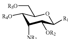
Scaffold W8 derived from H-9
