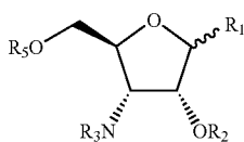
Scaffold W9 derived from J-4
