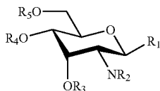
Scaffold W7 derived from G-4
