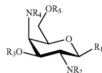
Scaffold W1 derived from A-6
