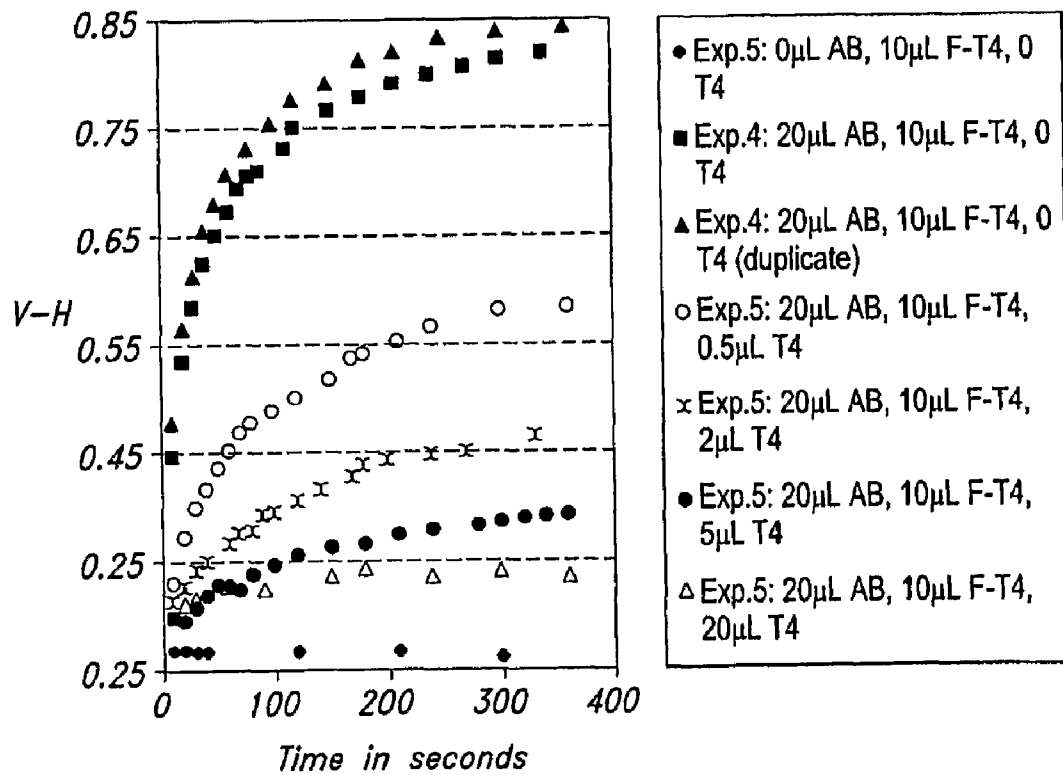
Competitive Inhibition by T4 of anti-T4/F-T4 System
