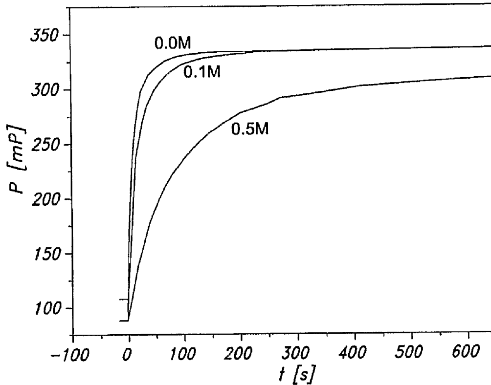
Effects on a fluorescein-T4/anti-T4 system using differing concentrations of additive sodium chloroacetate combined with 4.75% 2-propanol.
