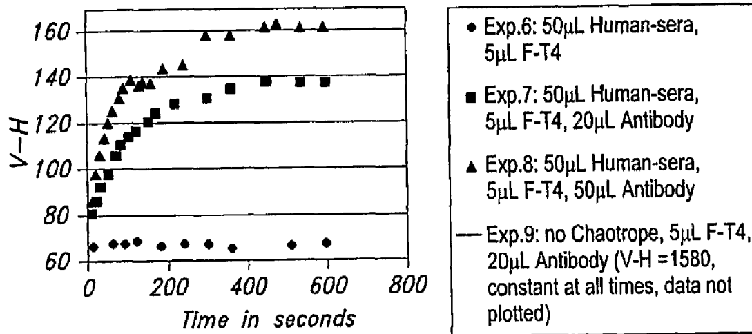
Additive Effects on Specific and Non-specific Binding
