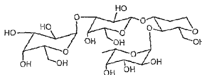
Glycomimetic 1
