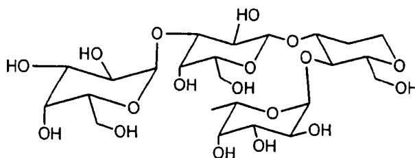
Glycomimetic 1
