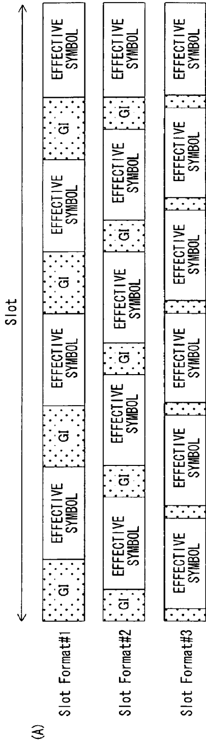
EXAMPLE OF SLOT FORMAT USED FOR SYSTEM (EFFECTIVE SYMBOL LENGTH IS CONSTANT)
