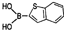
benzo[b]thiophene-2- boronic acid (5ZBTH2B)
