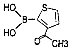
5-acetylthiophene-2- boronic acid (5ACTH2B)
