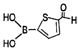
3-formylthiophene-2- boronic acid (3FTH2B)
