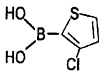
5-chlorothiophene-2- boronic acid (5CLTH2B)
