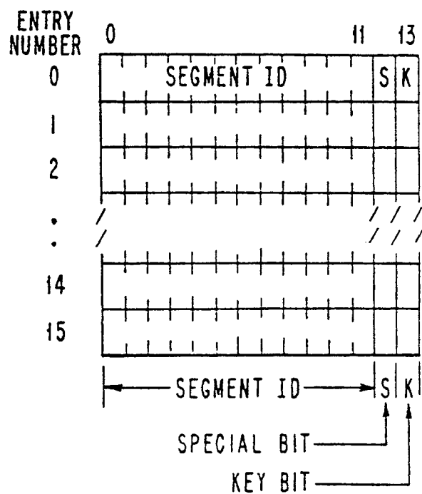
SEGMENT REGISTERS
