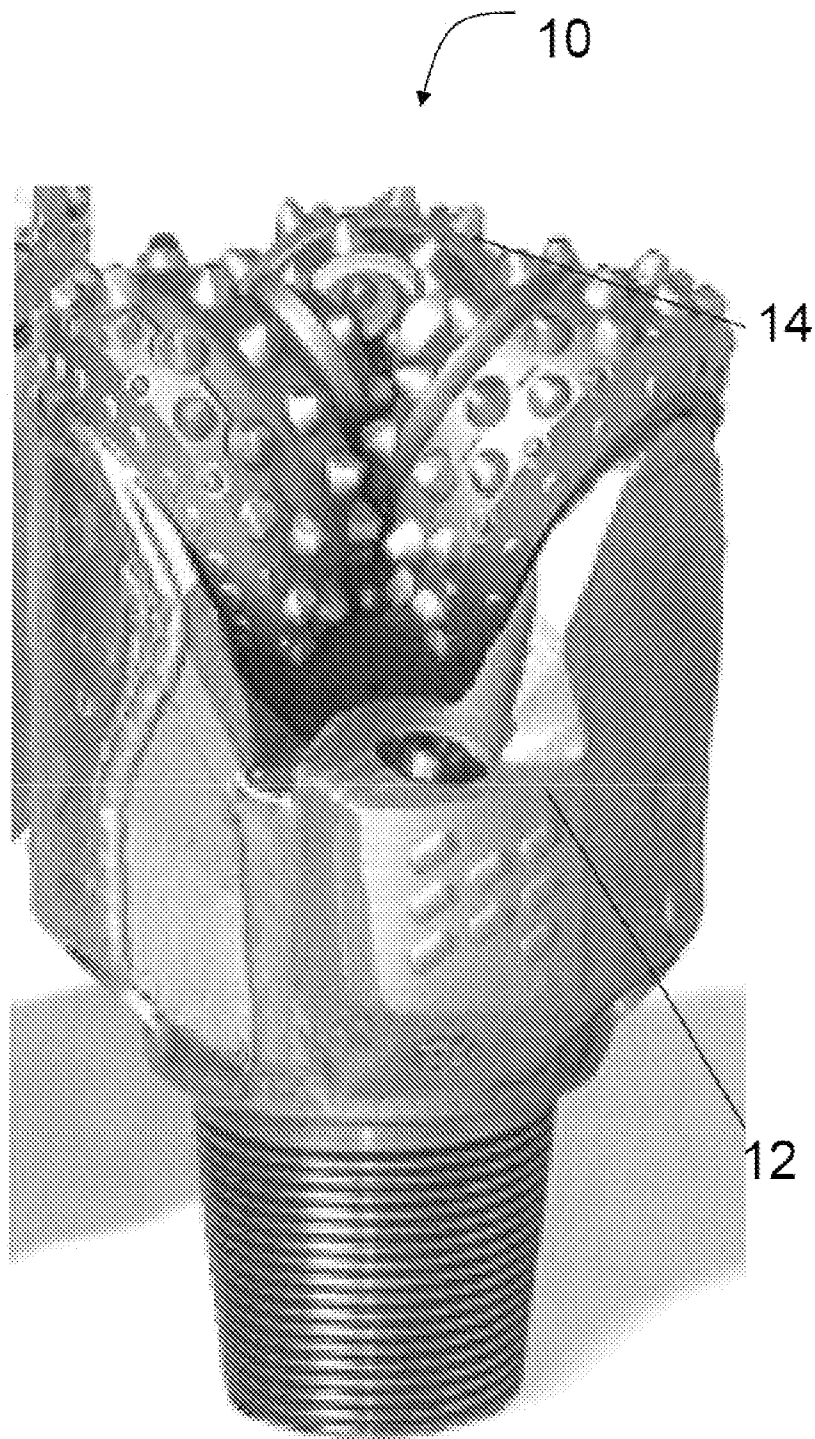
Figure 1 Prior Art
