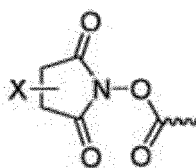
[Chemical Formula 30]
