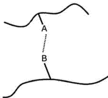
Schematic scheme for reaction (II)
