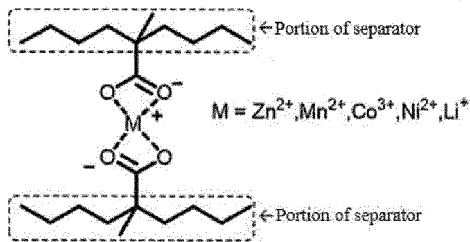
[Chemical Formula 53]
